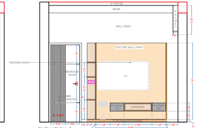
ELEVATION-C
