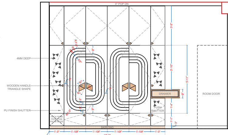
ELEVATION-B
