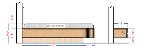
BED+SIDE UNIT SIDE ELEVATION
