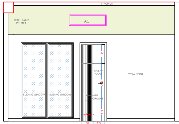
ELEVATION-D
